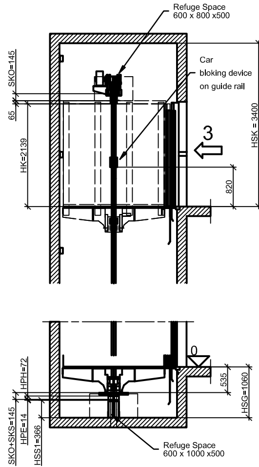
Car vertical Section: 1:50
