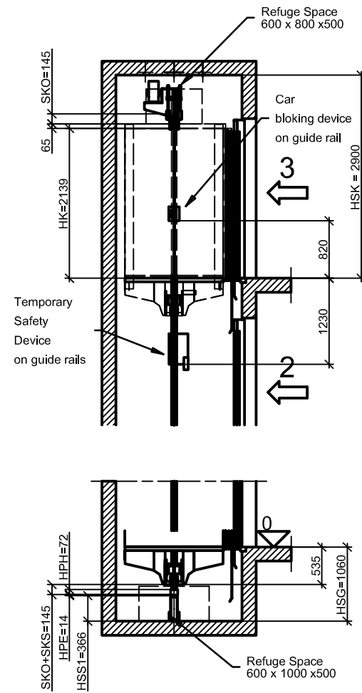
Car vertical Section: 1:50
